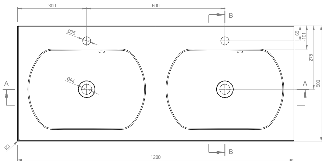
Bottom view
