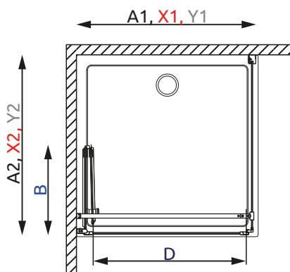
Balos kabin Variant L
